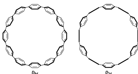
Scheme 5. Two optimized structures of [12]CPP.
